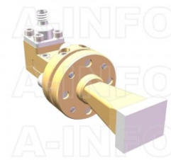
LB-10-15-C-1.0FSPO Standard Gain Horn Antenna 75-110GHz 15dB Gain 1.0mm Female
